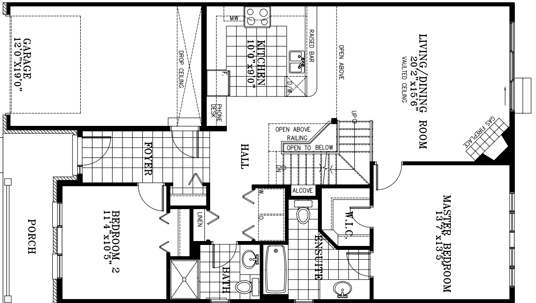
GROUND FLOOR PLAN B - ELEVATION 'B' ONLY 1183 sq. ft.
