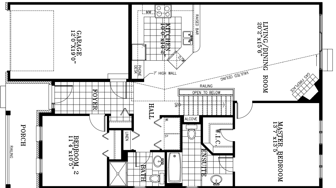
GROUND FLOOR PLAN A - ELEVATION 'A' ONLY 1183 sq. ft.
