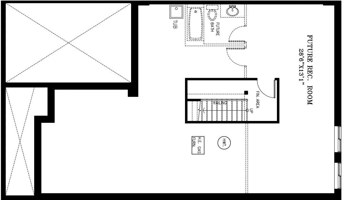
BASEMENT FLOOR PLAN A - ELEVATION 'A' ONLY FUTURE REC. ROOM 370 sq. ft.
