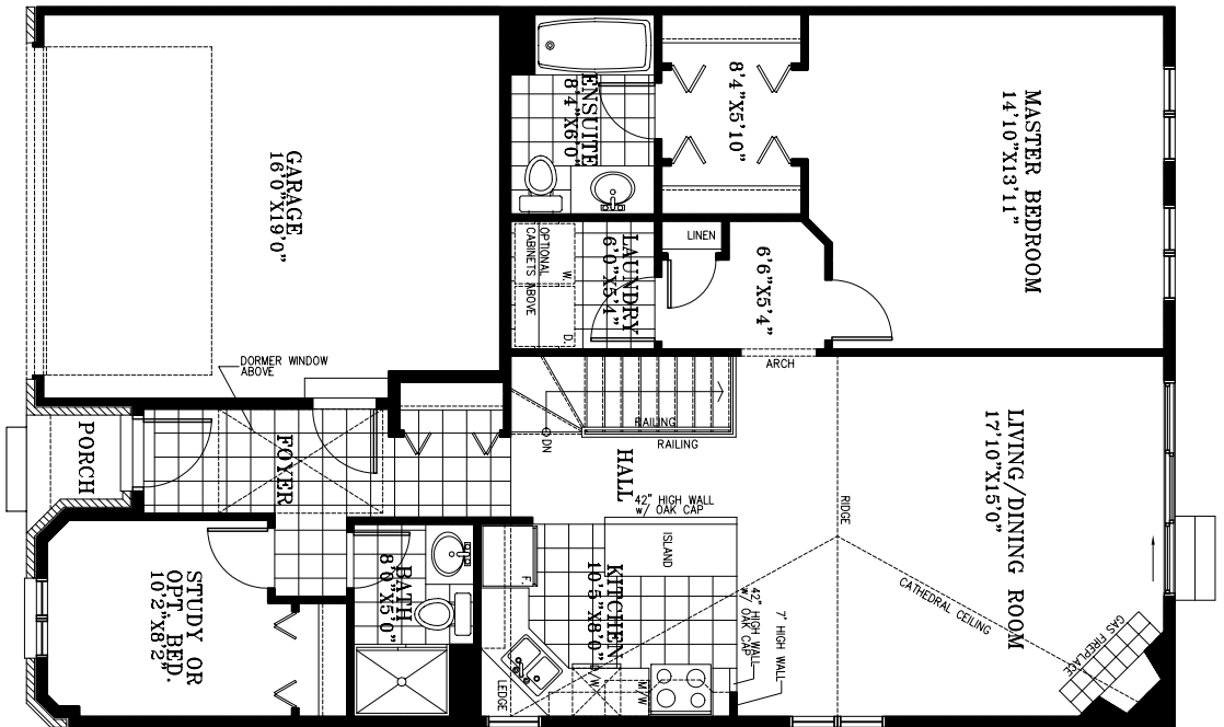
GROUND FLOOR PLAN 1099 sq. ft.
