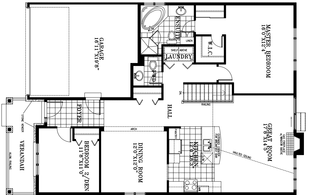
GROUND FLOOR PLAN - ELEV. 'A' 1265 sq. ft.
