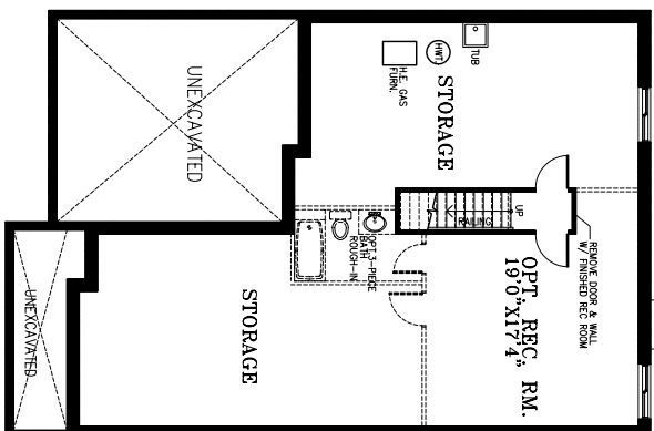
BASEMENT FLOOR PLAN 306 sq. ft. opt. fin. rec. room
